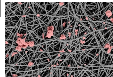
Nanofibers Defects
